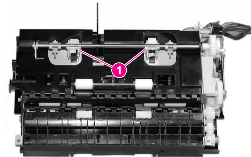
Figure 6-21 Remove the cassette (tray 2) pickup rollers
