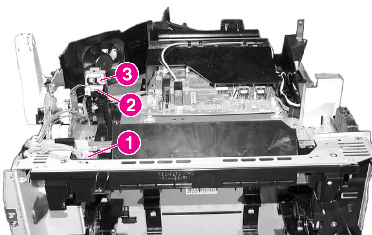
Figure 7-22 Fuser sensors and output bin full sensor
