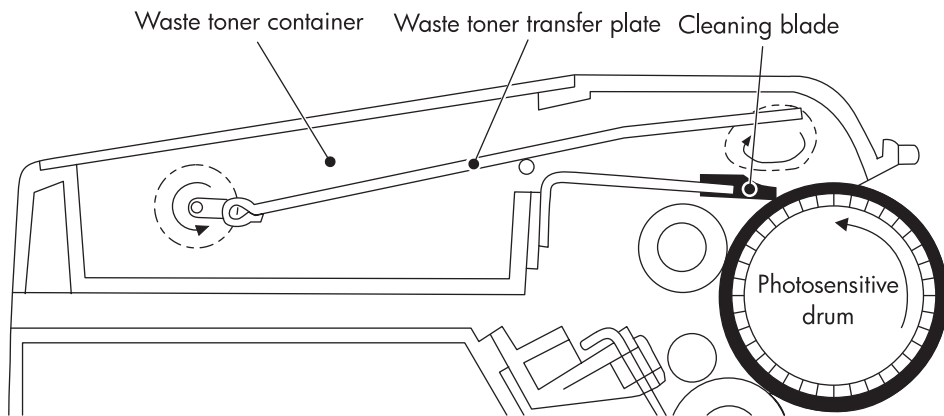
Figure 5-29 Drum cleaning
