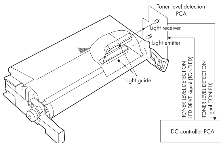
Figure 5-17 Toner-level detection
