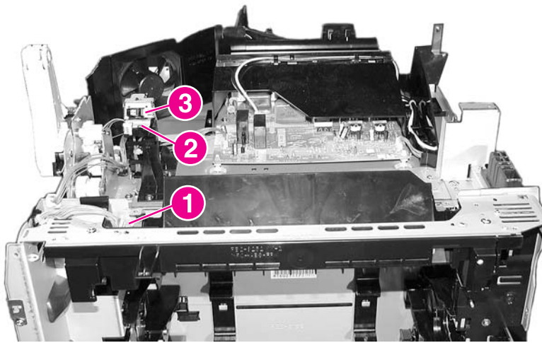
Figure 7-36 Fuser sensors and output bin full sensor
