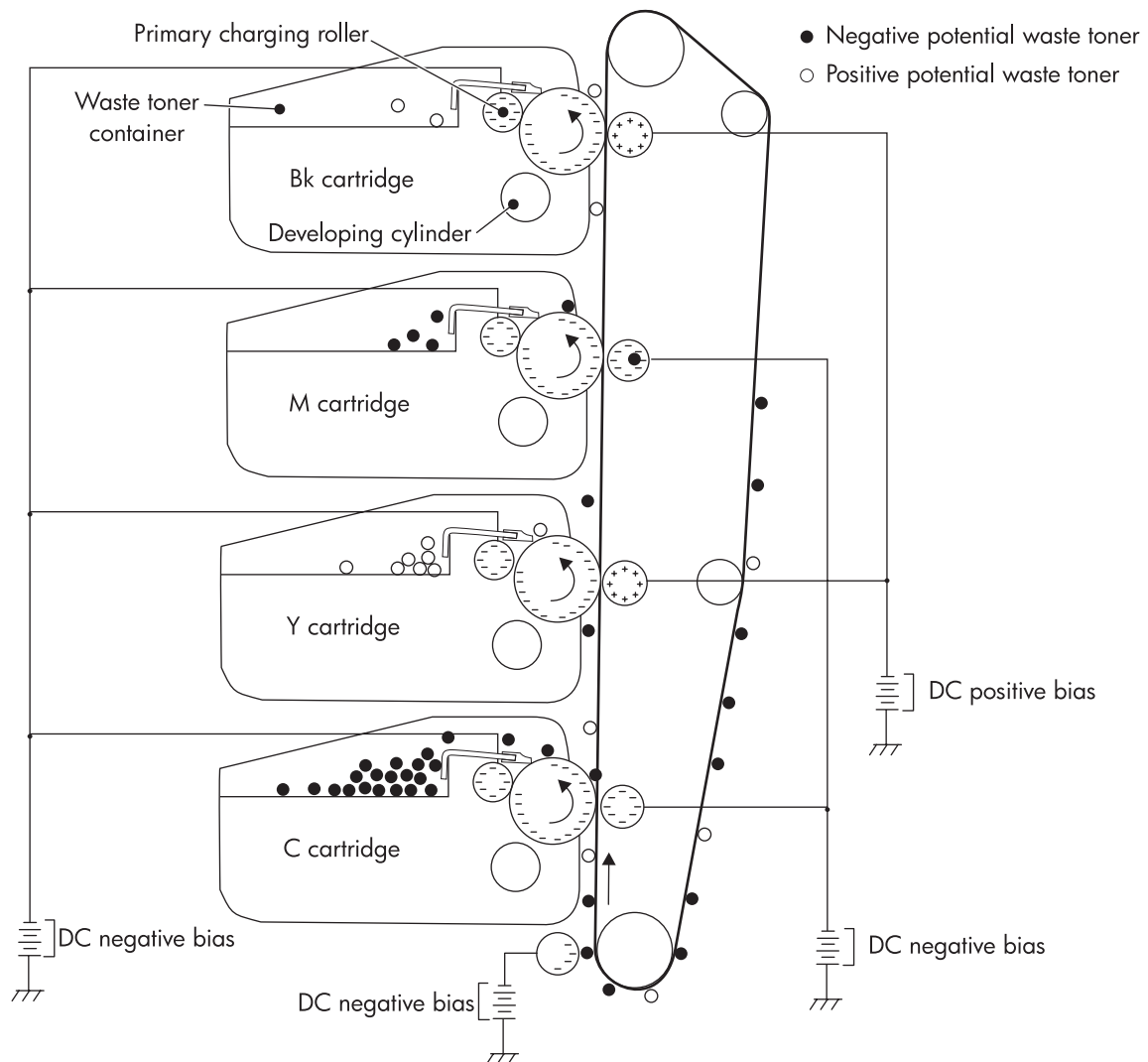
Figure 5-28 ETB cleaning
