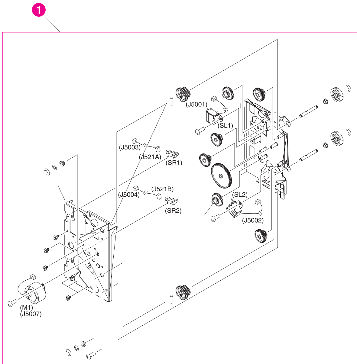
Figure 8-22 2 x 500-sheet feeder paper pickup drive assembly (HP CLJ 4650 models only)
